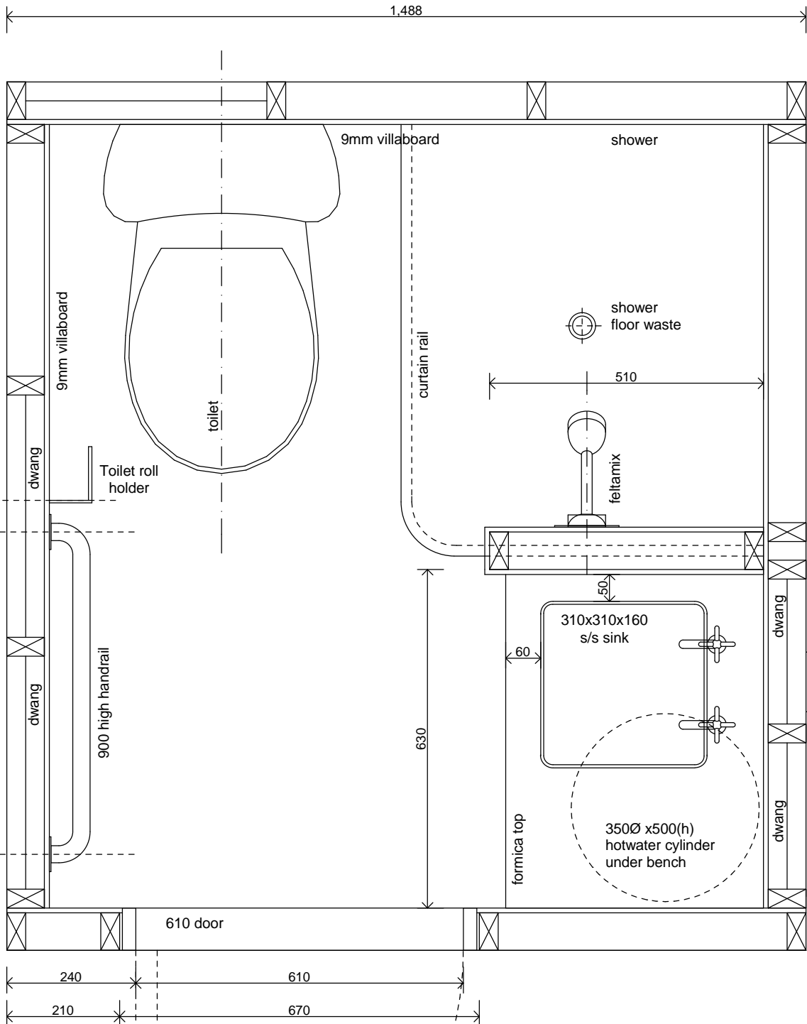
ENSUITE FLOOR PLAN SCALE 1:10
